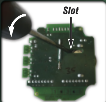
7. With a screwdriver lever the battery out through the slot in the PCB
